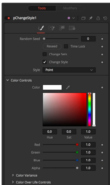
The pChange Style controls
