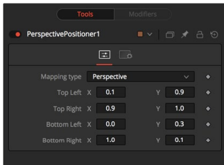
The Perspective Positioner Controls tab
