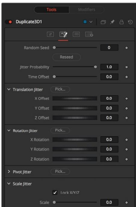
Duplicate 3D Jitter tab
