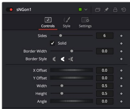
The sNGon Controls tab
