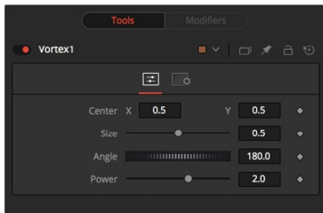
The Vector Distortion Controls tab
