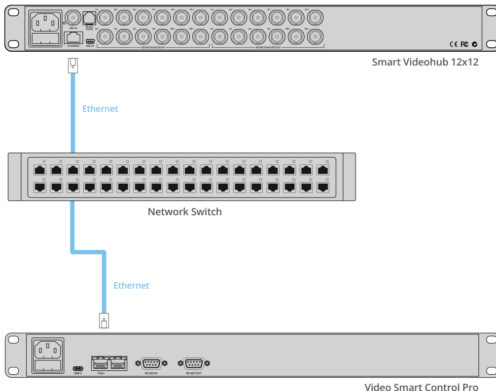
Videohub Smart Control Pro connected to a Smart Videohub 12x12 via an Ethernet Network Switch.
