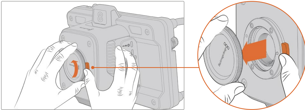
Press the lens release button and rotate the dust cap counterclockwise until it is released from the mount
