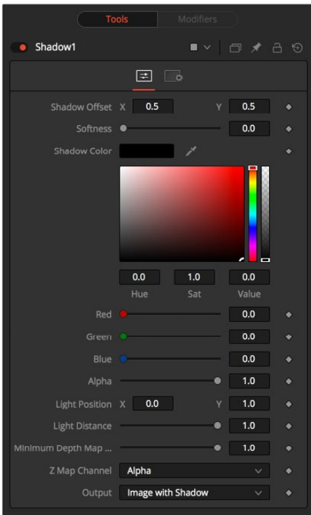
Shadow node controls
