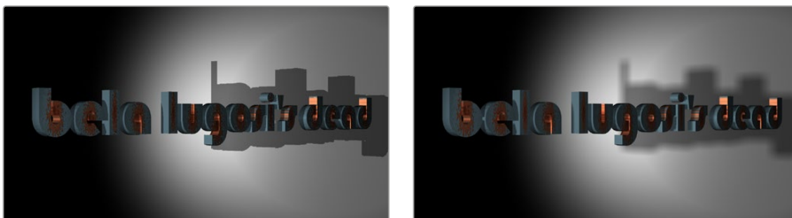
When the Renderer3D node "Renderer Type" drop-down is set to OpenGL Renderer, you cannot render soft shadows or excessively large textures (left). When the Renderer3D node "Renderer Type" drop-down is set to Software Renderer, you can render higher-quality textures and soft shadows (right).
