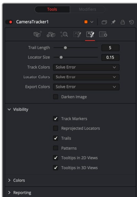
The Camera Tracker Options tab
