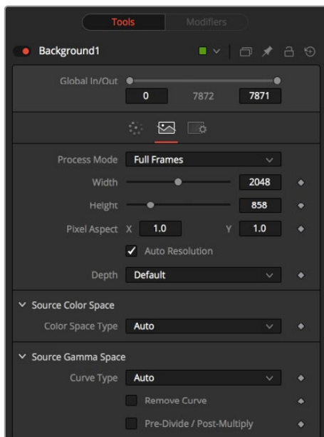
Background node Image tab
