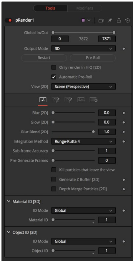
The pRender controls
