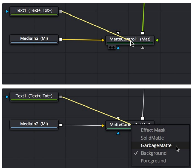
Option-dragging a node connection to drop onto another node exposes a node input menu
