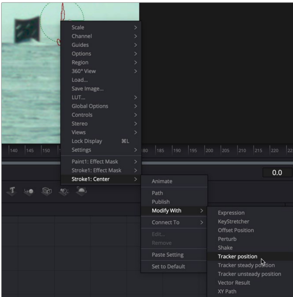
Right-clicking over the Stroke's Center control in the view allows you to apply a tracker modifier
