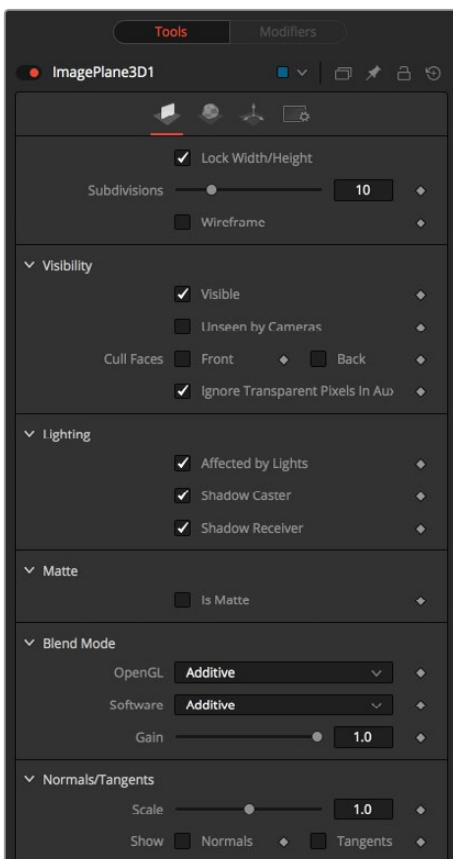
Image Plane 3D controls
