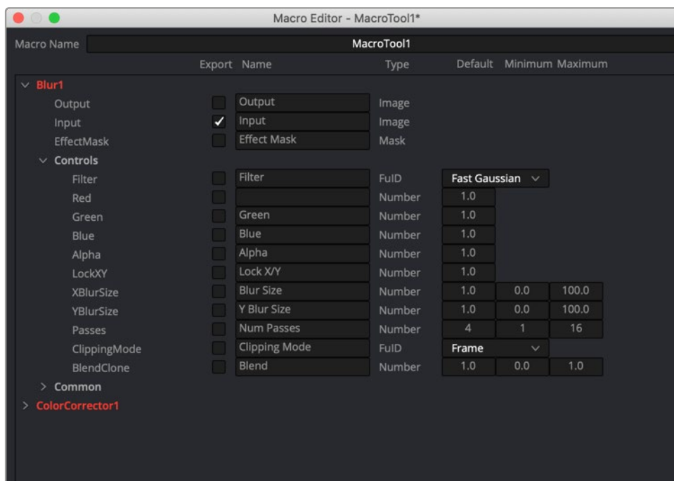
The macro editor with a Blur node and Color Corrector node.
