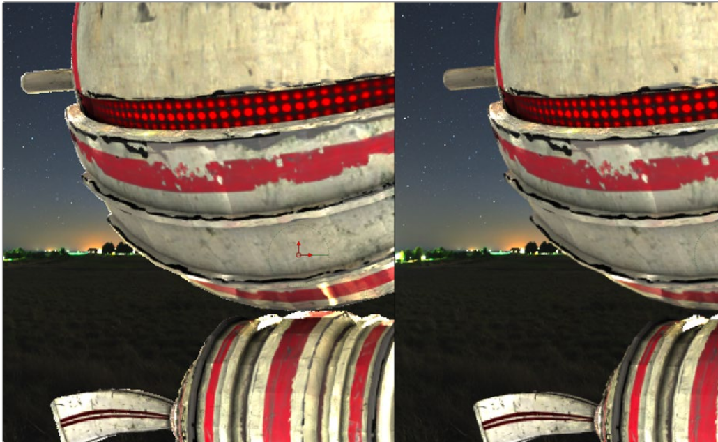
Nonpremultiplied edges in an additive Merge (left) and premultiplied edges in an additive Merge (right)
