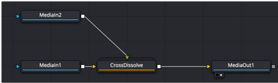
The Cross Dissolve node tree in Fusion.
