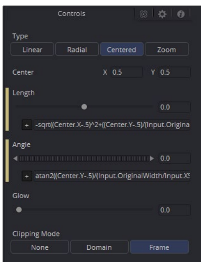
Directional Blur controlled by the Center's position
