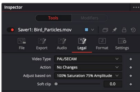
Saver Legal tab
