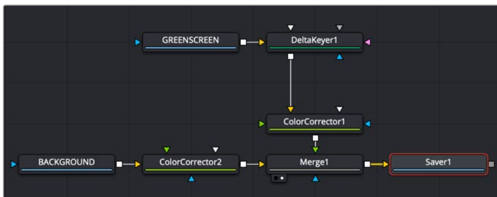
Saver node added to the end of a node tree to render the composition
