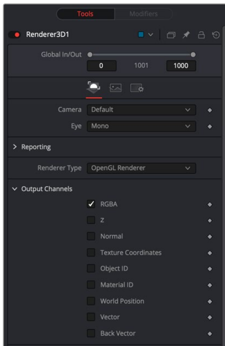
Render 3D Open GL controls
