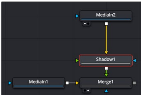
A Shadow node is generated from the MediaIn2 and shown over MediaIn1
