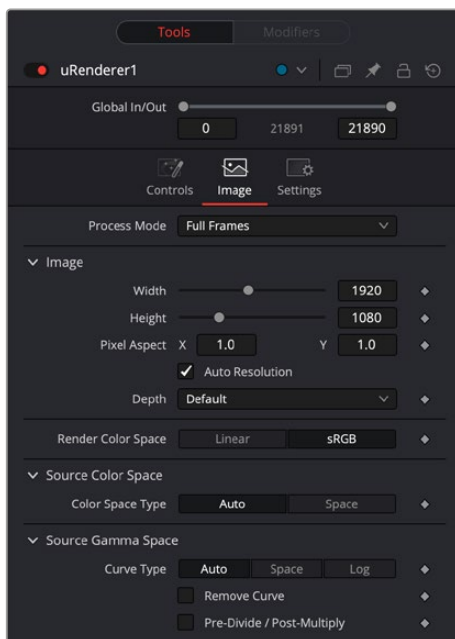
USD Renderer Image controls
