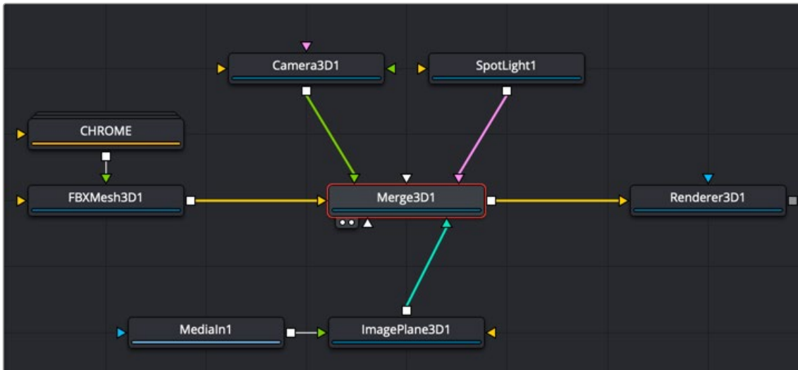
Merge 3D with a connected Image Plane, FBX Mesh object, SpotLight, and camera
