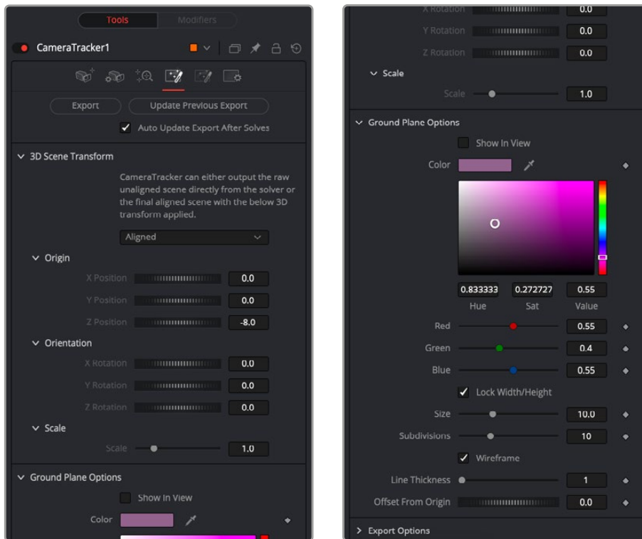
The Camera Tracker Export tab
