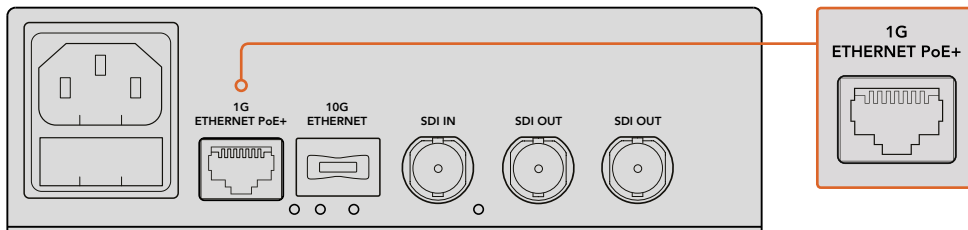
Plug HD video to and from your network via the 1G Ethernet connector
