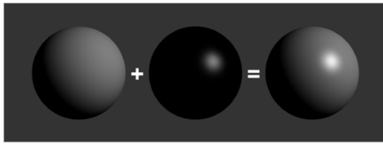
Three spheres, left to right: diffuse only, specular only, and combined
